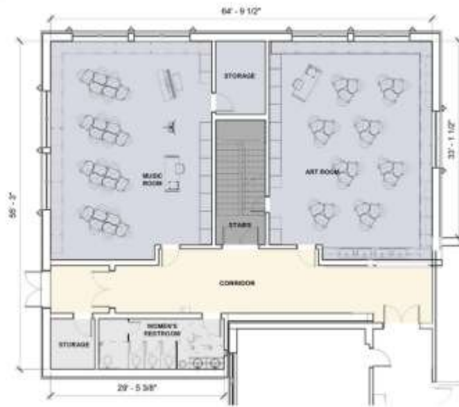
BUILDING ADDITION LEVEL 1 - ART & PERFORMING ARTS SPACES
